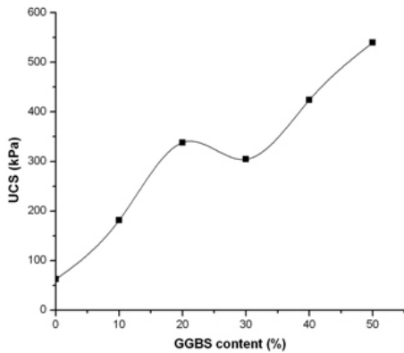
Fig. 2 Variation of UCS of BC soil with GGBS content
