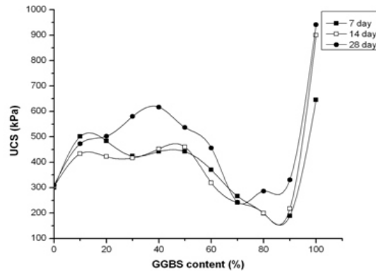
Fig. 3 Variation of UCS of Fly ash with GGBS content
